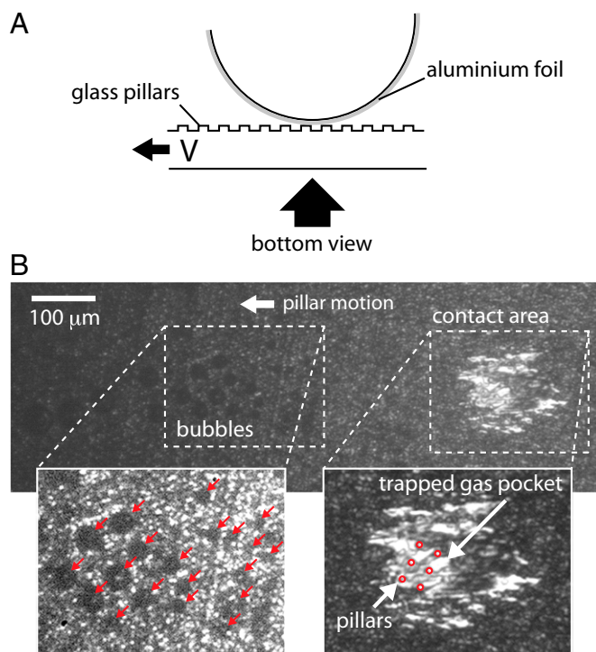
Fig. 6. (A) Schematic of the setup: a transparent glass surface covered with micropillars is rubbed against a bead covered with aluminium foil ( F = 7 \times 10^{-2} N, V = 4.7 mm·s -1 ). (B) Bottom view of the experiment through a microscope. Gas pockets are trapped between the two solids in the contact area, and microscopic gas bubbles (red arrows) are observed downstream. The spacing between the pillars, their diameter, and their height are 10, 9, and 0.3 µm, respectively.
