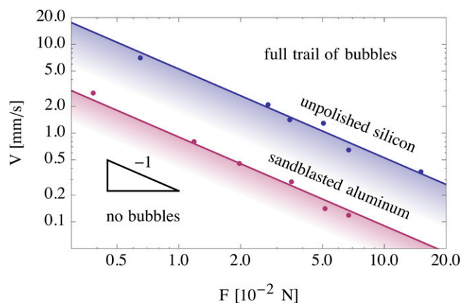
Fig. 4. Comparison between the force–velocity thresholds for unpolished silicon and sandblasted aluminum submerged in ethanol at 70 °C and having similar roughness \mathcal{R}_a \sim 0.5 \mu\text{m} . The solid lines correspond to FV = \text{const} . In the shaded area, we still observe a partial bubble trail (Fig. 3).
