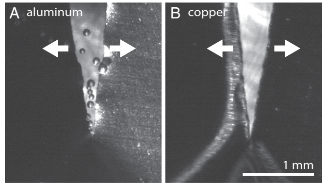
Fig. 9. Snapshots of the tearing of thin foils of (A) aluminum and (B) copper submerged in ethanol at around 78^\circ\text{C} . The foils are 12.0 and 12.5\ \mu\text{m} thick, respectively, and the two sides of the foil are torn apart with a velocity of about 9\text{ mm}\cdot\text{s}^{-1} . For aluminum, bubbles form at the tip of the tear, whereas for copper no bubbles form.
